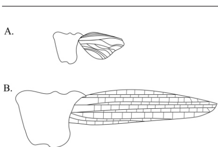
Figure 3. Lateral view of the basic venation of an acridid wing. "A" represents the basic venation of a fifth instar wing pad. "B" represents the basic venation of an adult wing. Please note, the nymphal wing pad venation curves downward while the adult wing venation runs parallel to the body. Image Credit: Erika Rodbell
