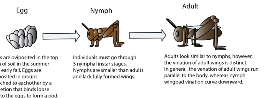
Figure 2. The grasshopper life cycle is an incomplete life cycle featuring egg, nymph, and adult life stages. Image Credit: Erika Rodbell
